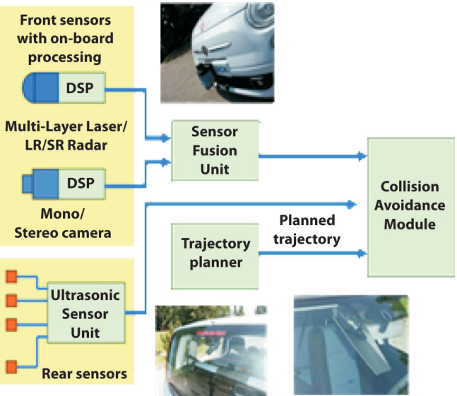
Obstacle detection system
