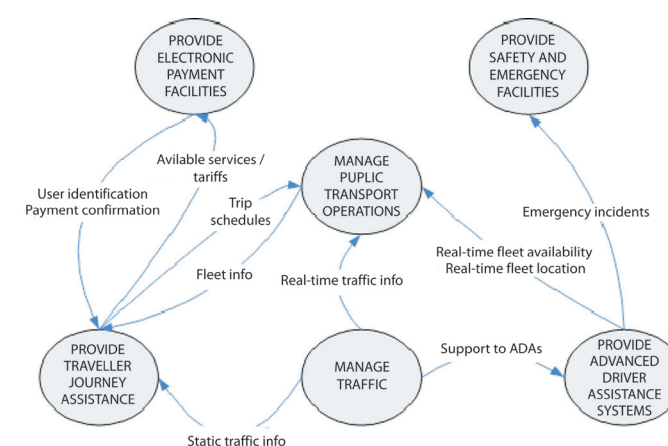
Architecture and information flow: Functional architecture example
